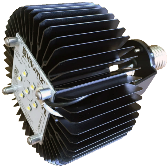
DZ3X (shown with vertical mount)
